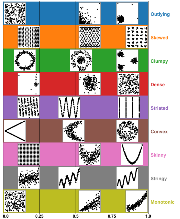
Fig. 9. Some example scatterplots and their measures [19]. In each row, the scatterplots with a low score on the associated measures are on the left while the scatterplots with a high score on the associated visual features are on the right.
