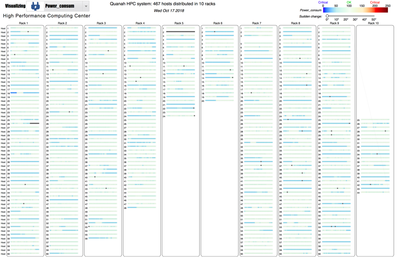
Fig. 4. Visualizing power consumption on Wednesday, October 17, 2018, of the 467-node Quanah cluster at Texas Tech University.
