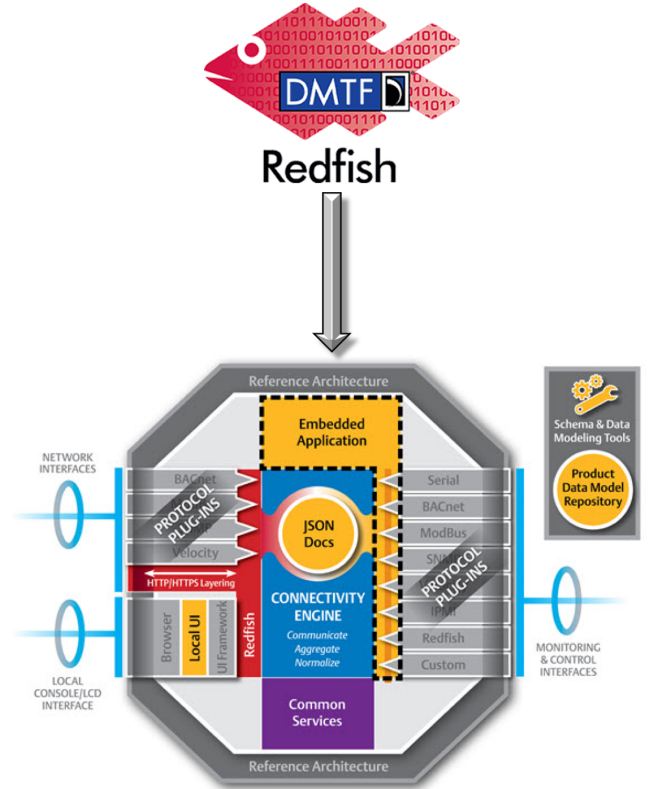
Fig. 1. Redfish reference architecture [2].
