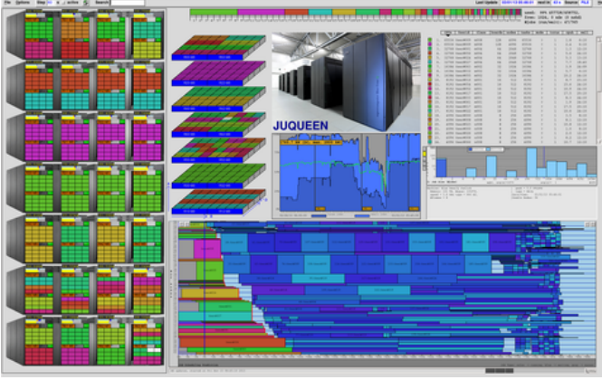
Fig. 2. Main window of LLview [3]: Graphical monitoring of batch system controlled cluster.
