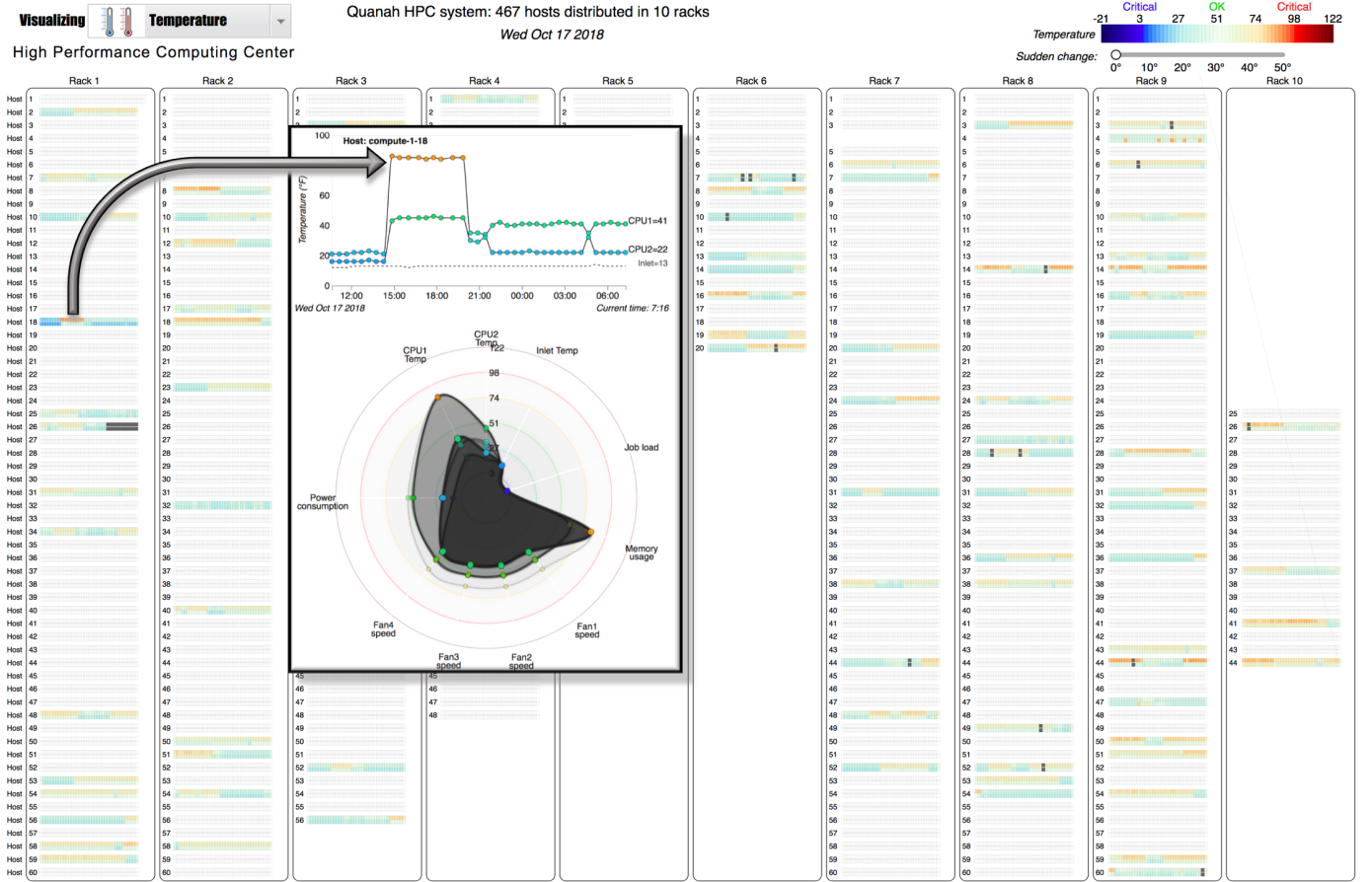
Fig. 5. Visualizing CPU temperature on Wednesday, October 17, 2018 of the 467-node Quanah cluster. Hosts experiencing a sudden temperature increase of 25 degrees in 3 minutes.
