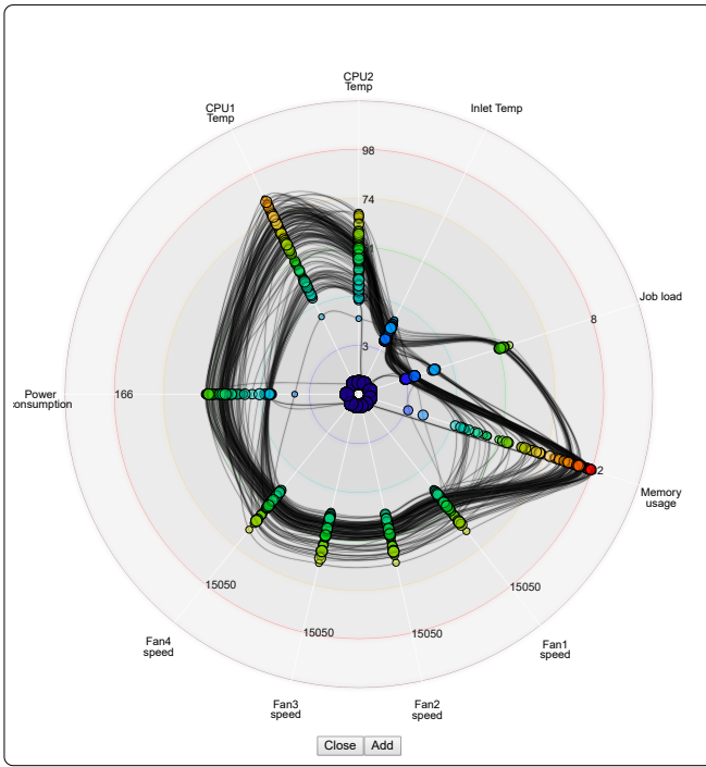
Fig. 7. Visualizing multidimensional health status at 2 pm on Wednesday, October 17, 2018, of the 467-node QuanaH cluster at Texas Tech University.
