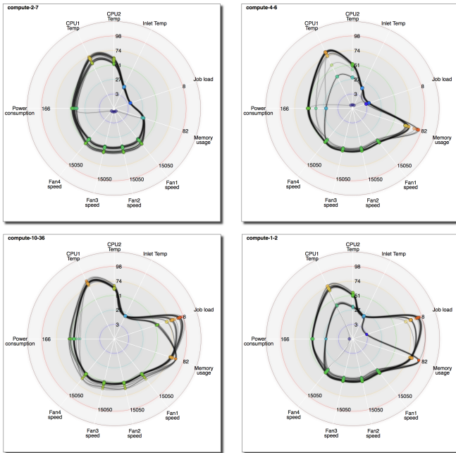
Fig. 6. Visualizing multidimensional health status of four different hosts in the data center.
